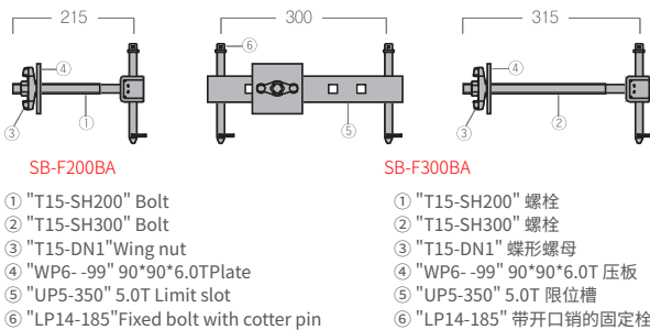
Formwork and support fixed bolt 模板与支撑固定螺栓
