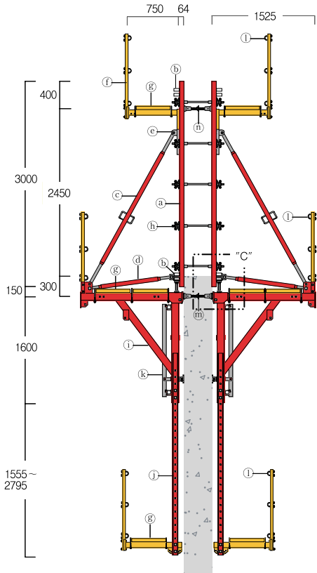
"FCB-1515BA" Double-side formwork hanging bracket system 双侧模板挂架系统
