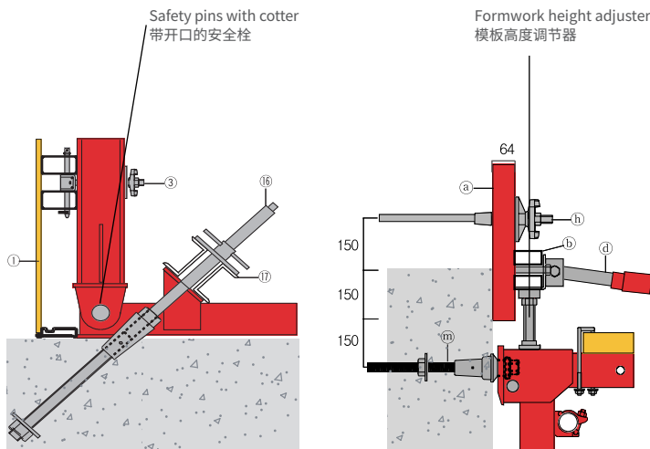
Detailed drawing "A" 详图 "A"
