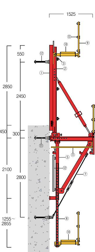
"SFC-1521BA" Single-side formwork hanging bracket system 单侧模板挂架系统
