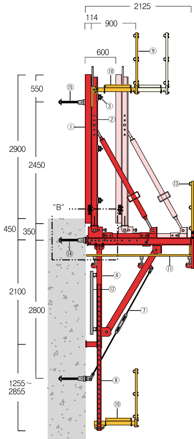
"SFC-2121BA" Single-side formwork hanging bracket system 单侧模板挂架系统
