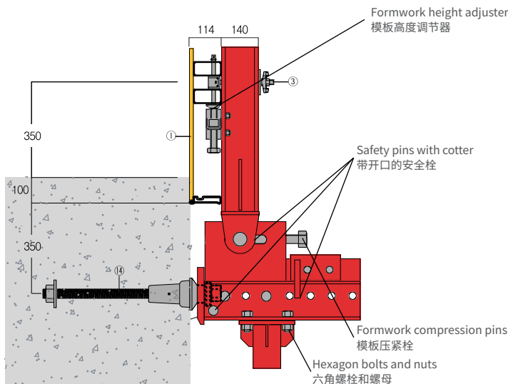
Detailed drawing "B" 详图 "B"
