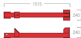
SFC-SB 1500 Vertical support benchmark beam 纵支撑基准梁
