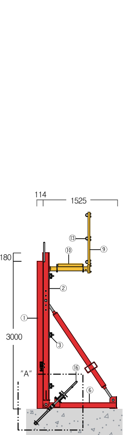
"SFC- 1500A" Unilateral force system 单侧强力系统
